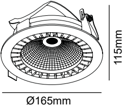
OPTIC LED
