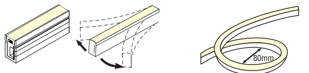
Minimum bending Ø80mm
