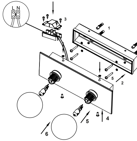
Ref. 63006 2 x G9 MAX. 28W no incl
