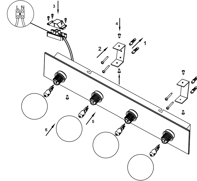
Ref. 63008 4 x G9 MAX. 28W no incl
